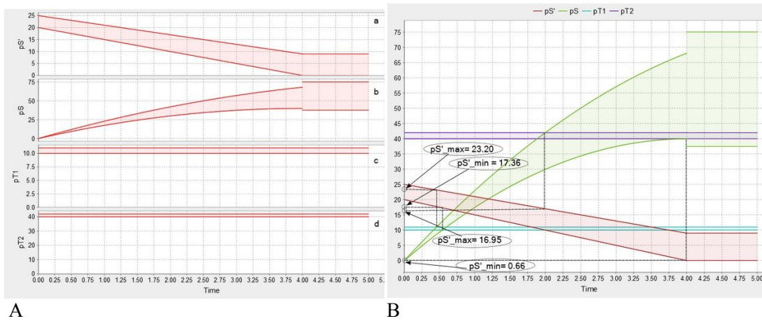
Figure 4: (A) Re-running the simulation shown in Figure 3(A) with enclosures, enables the automatic computation of the bounds of system behaviour; (B) Similarly to the method employed in Figure 3(B), we can determine the velocities at impact.
