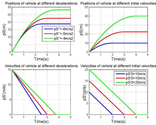
Figure 2: Instead of individual simulation traces to cover ranges of possible system behavior, enclosures allow us to automatically compute the upper and lower bound of any possible combination of the individual traces.
